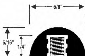
M-868-2 8/32 Insert
