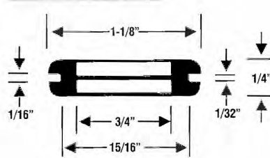
M-2196-W Solid Web
